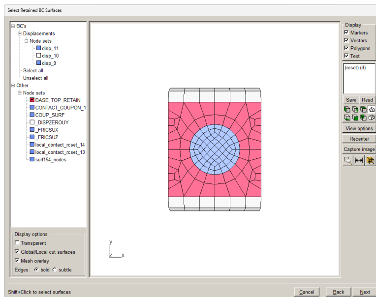
Figure 5.13 Mapped remeshed surface portion constrained by the retained surface mesh.
