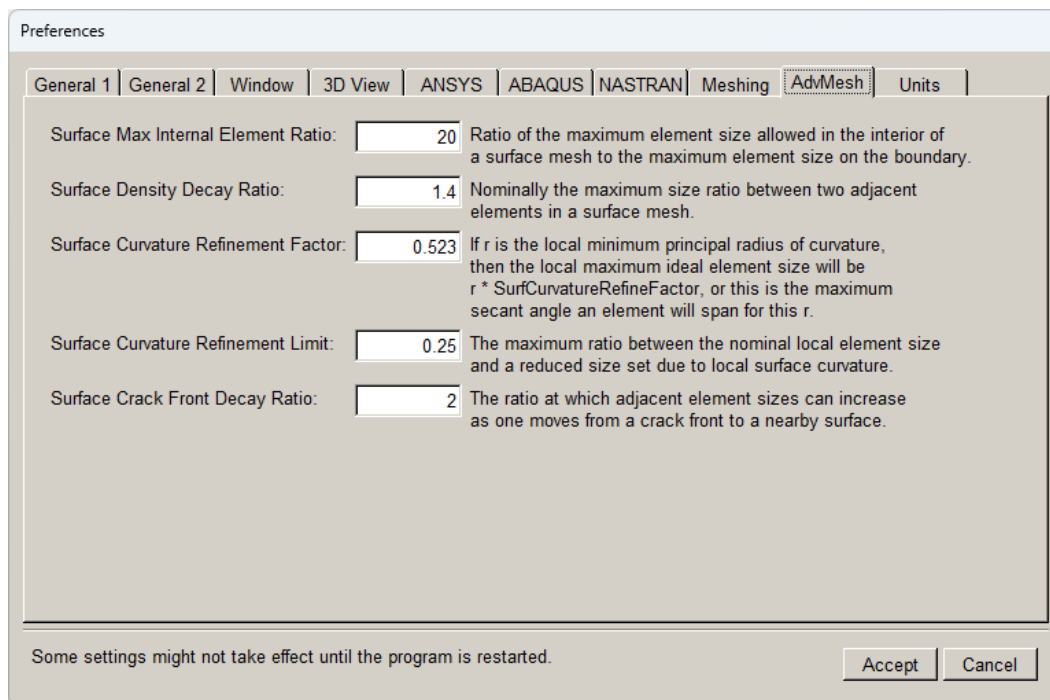
Figure 7.1 Advanced Meshing tab of FRANC3D Preferences dialog.
