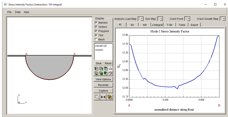
Figure 12.29 Mode I SIFs for the base-with-temperature model.
