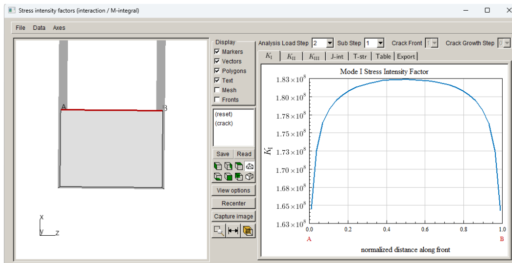
Figure 14.16c Mode I SIFs for load step 2.
