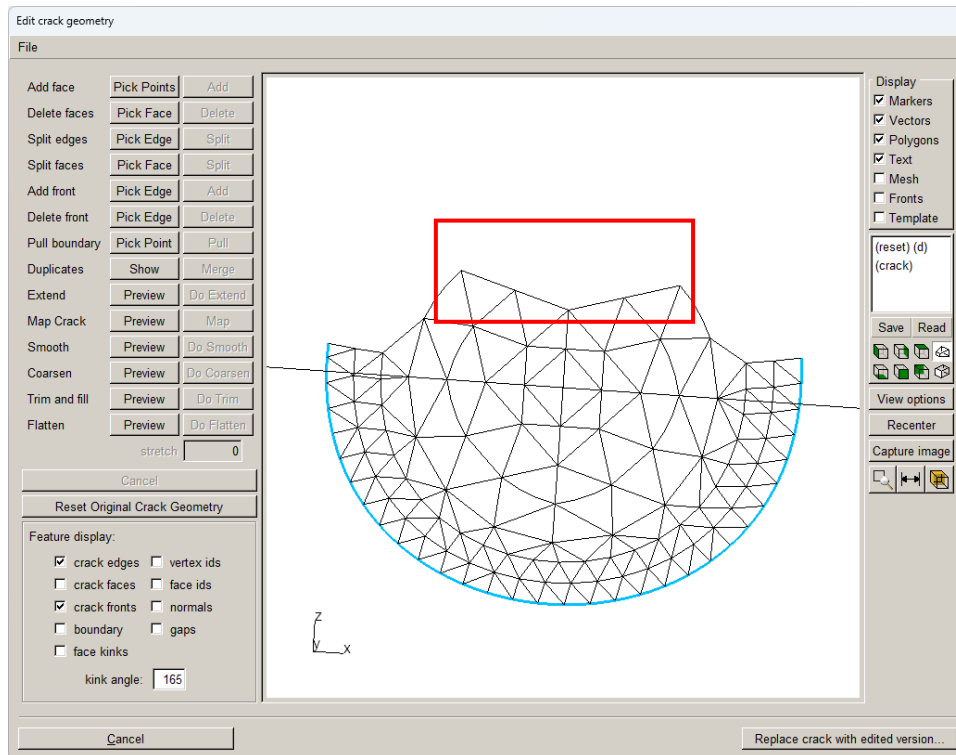
Figure 8.50b Faces are deleted.
