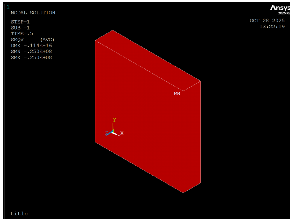
Figure 14.11a von Mises stress after applying initial stress in the elastic plate with all nodes constrained.
