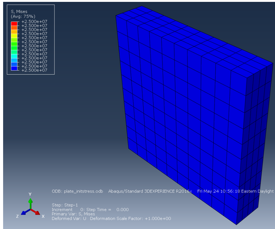
Figure 14.7a von Mises stress for load step 1 and frame 0 in the elastic plate with initial stress.
