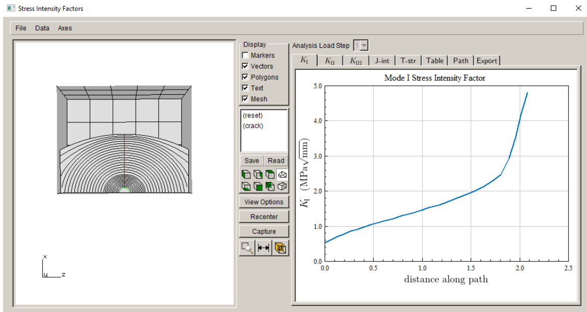
Figure 5.26 Complete SIF history.
