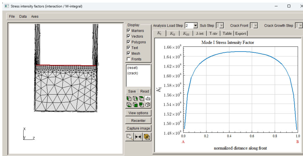
Figure 14.15b Mode I SIFs for load step 2.
