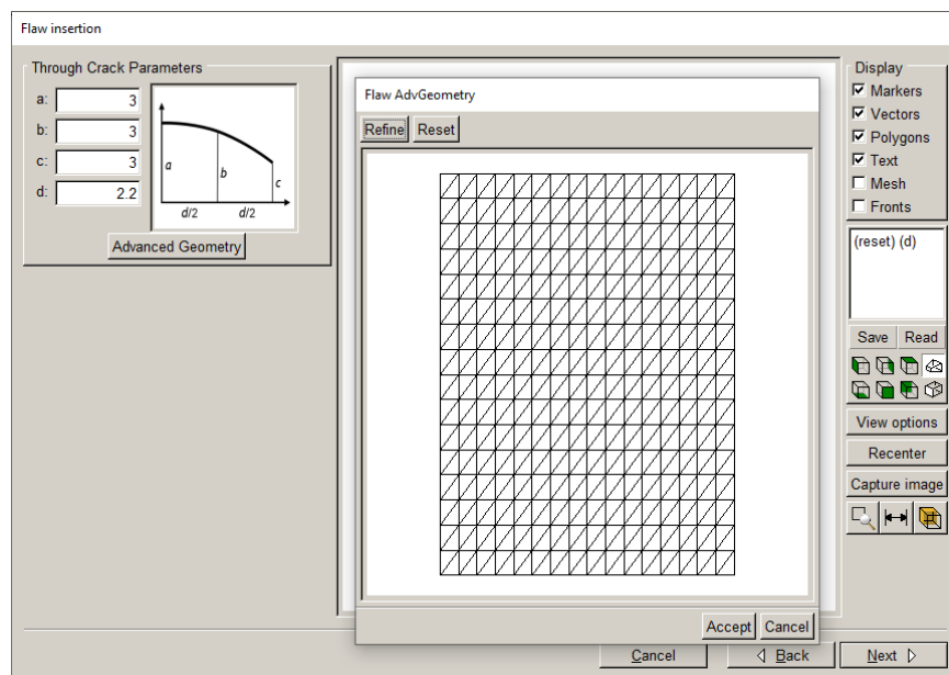
Figure 6.15 Refined geometry for an edge (through) crack with length of 3 units.
