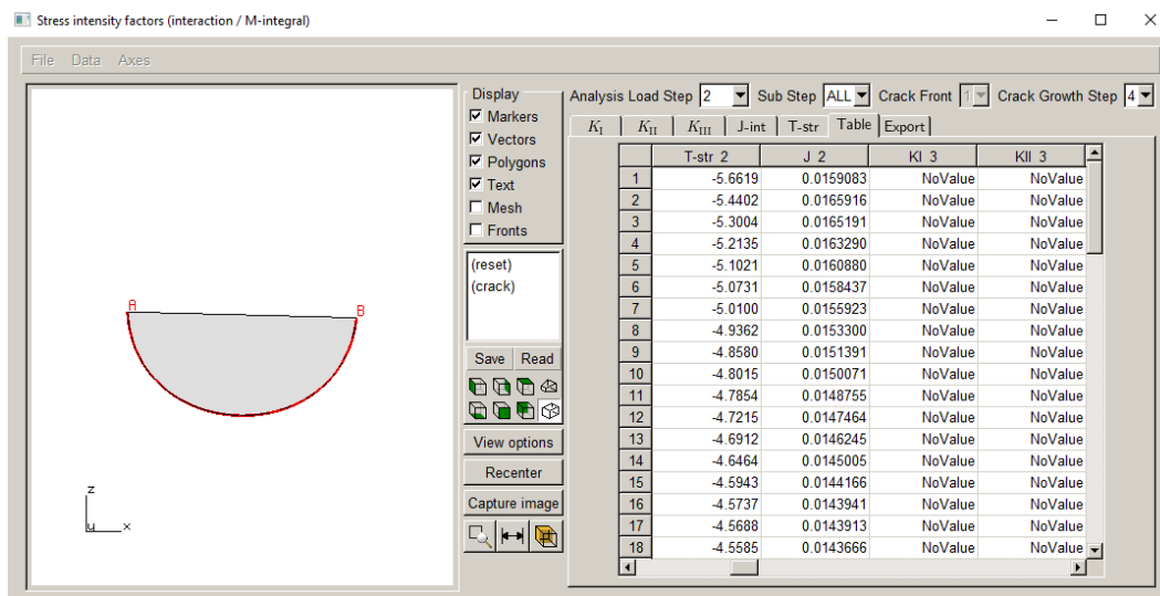
Figure 10.51 SIF table for load step 2 showing NoValue for substeps with missing results.
