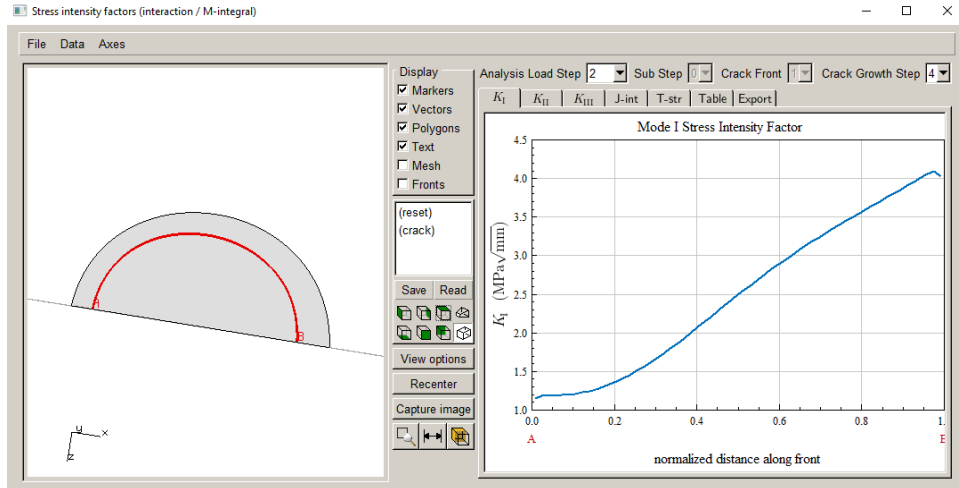
Figure 10.46 SIF plot for crack step 4 and load step 2.
