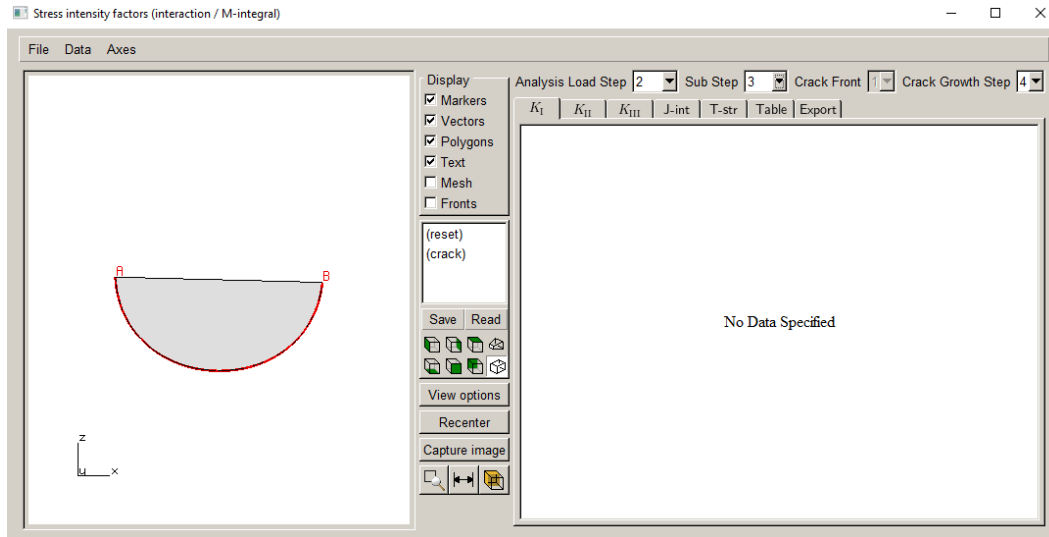
Figure 10.50 SIF plot for load step 2 for substep 3 with missing results.
