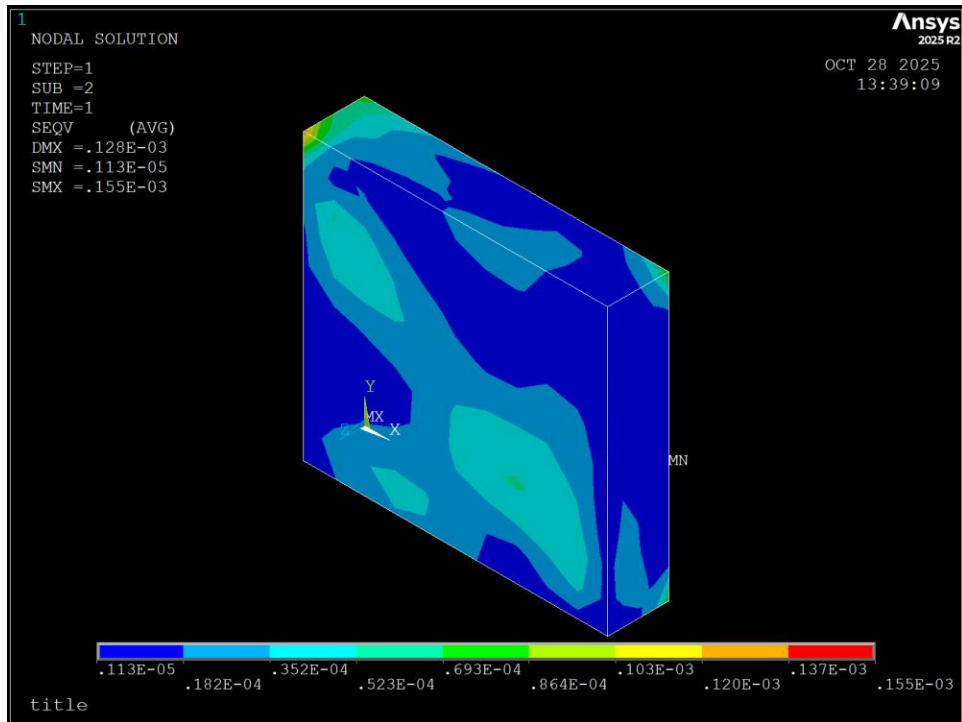
Figure 14.11b von Mises stress for load step 1 in the elastic plate with initial stress.
