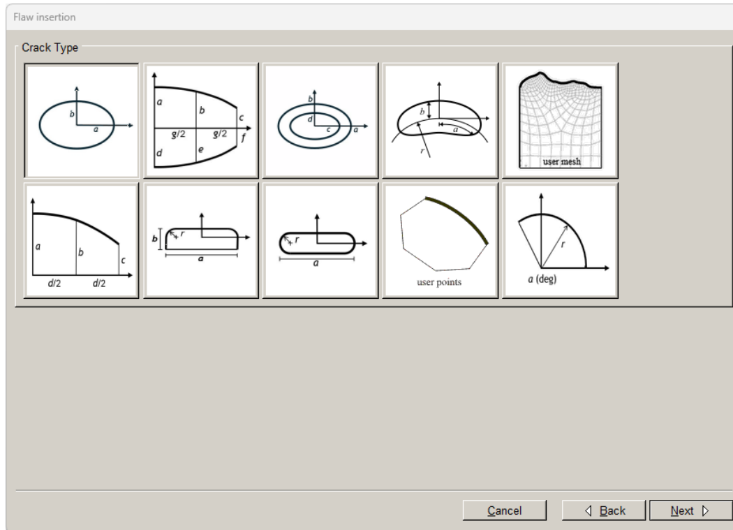
Figure 6.1 Crack shape library.
