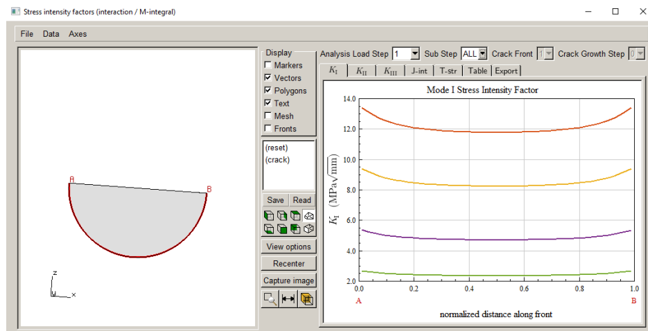
Figure 10.38 Mode I SIFs for all substeps of load step 1.
