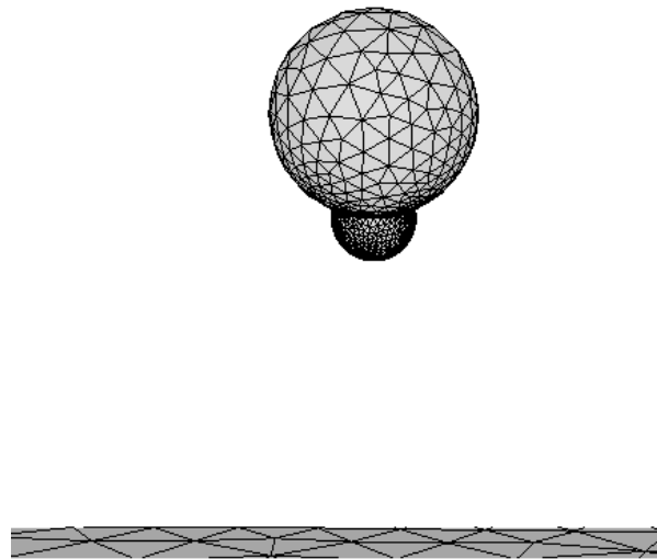
Figure 8.44 Surface mesh for a penny crack inserted into a void.
