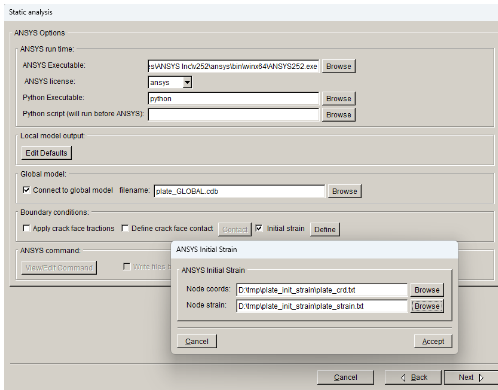
Figure 14.19 ANSYS initial strain dialog.
