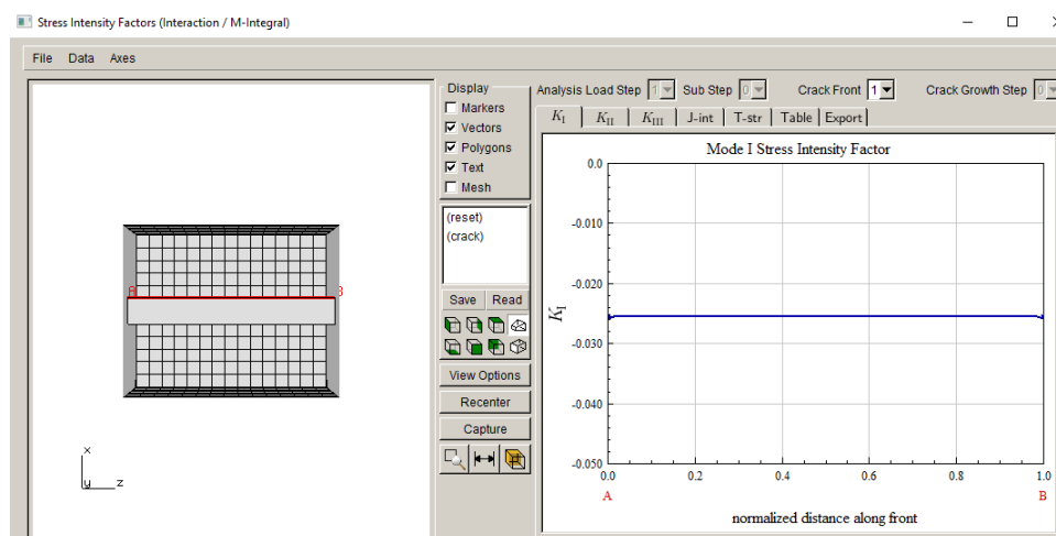
Figure 13.24 Mode I SIFs with modified template and default CFC using M-integral.
