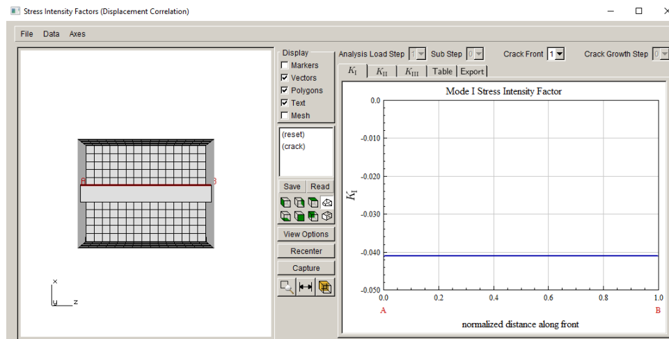
Figure 13.21 Mode I SIFs with crack front nodes included in bonded-CFC using DC.
