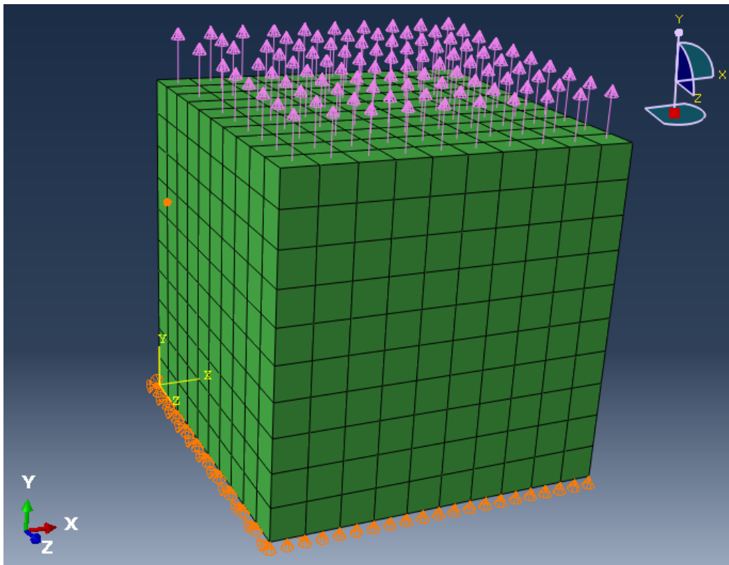
Figure 10.1 ABAQUS cube with tension on top surface.
