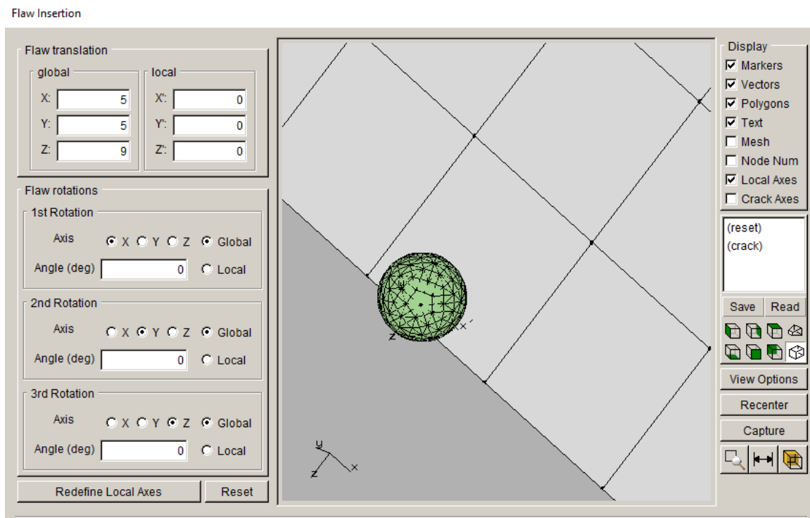
Figure 8.42 Interior void inserted into a cube.
