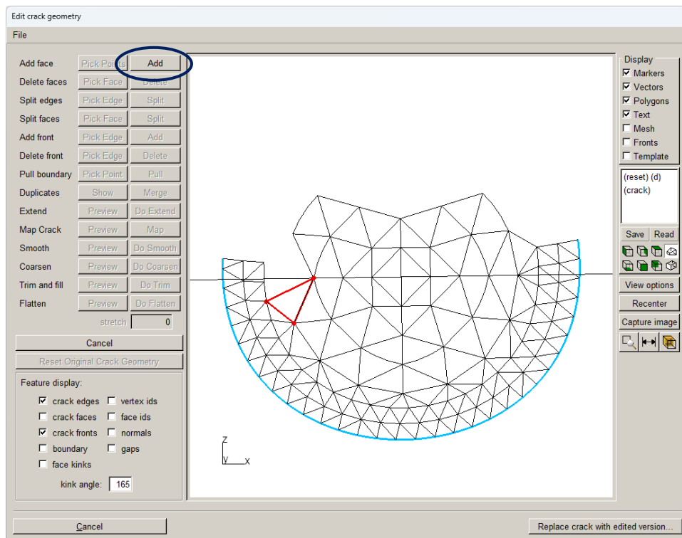
Figure 8.51b Face is added by clicking Add .
