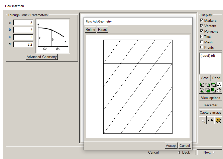
Figure 6.14 Geometry for an edge (through) crack with length of 3 units.
