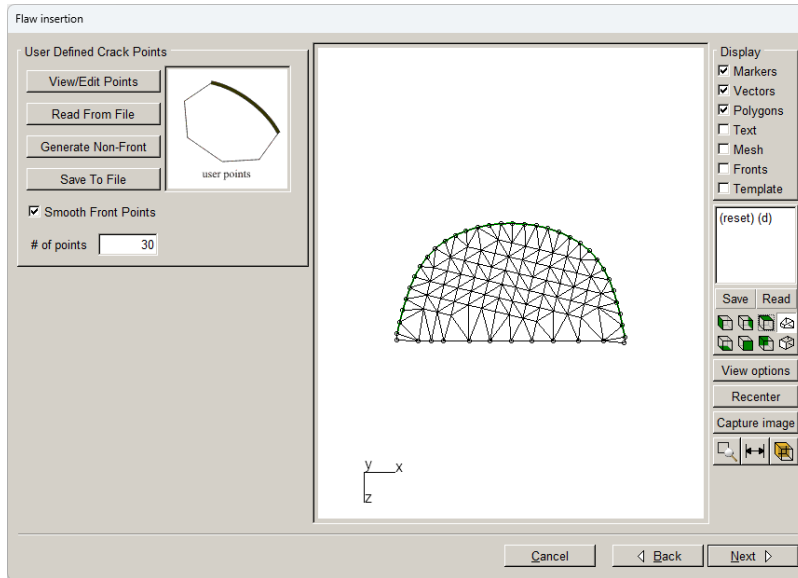
Figure 6.6 Additional non-front points produce a better triangulated surface.
