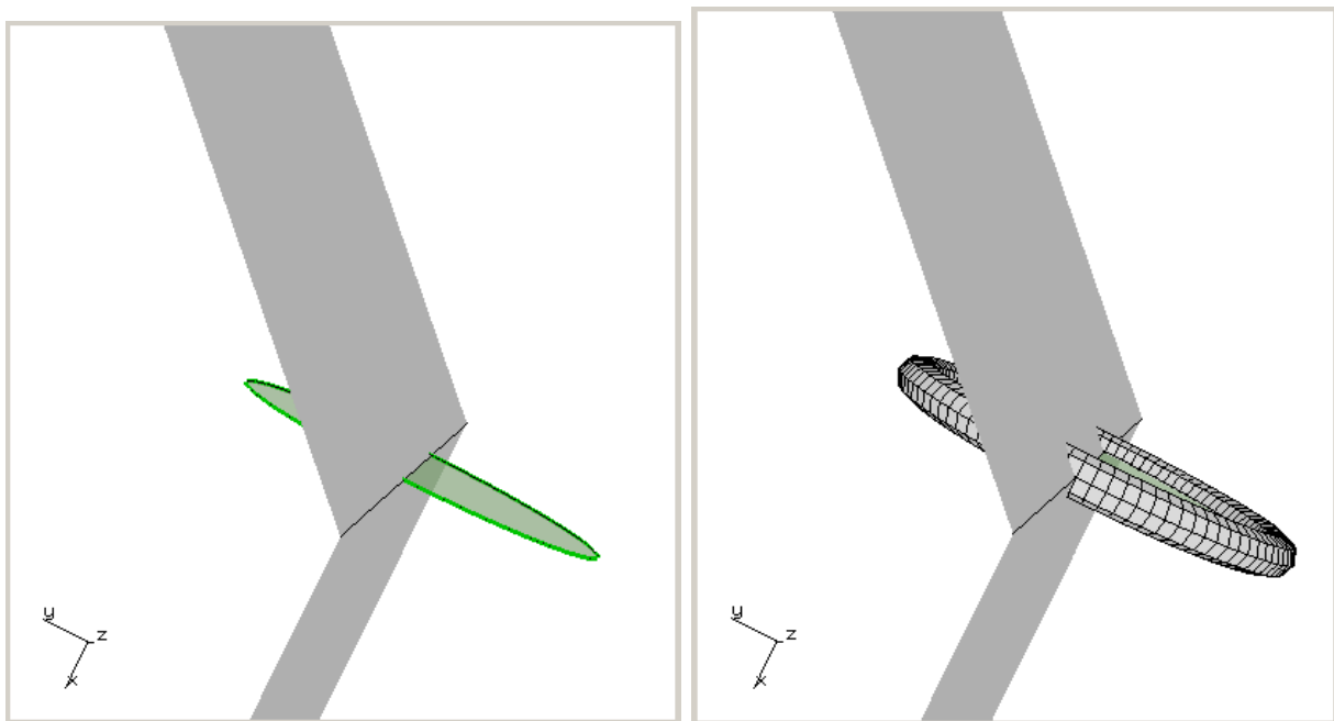
Figure 6.16 Crack inserted at a kink in the model surface – crack (left) and template (right).
