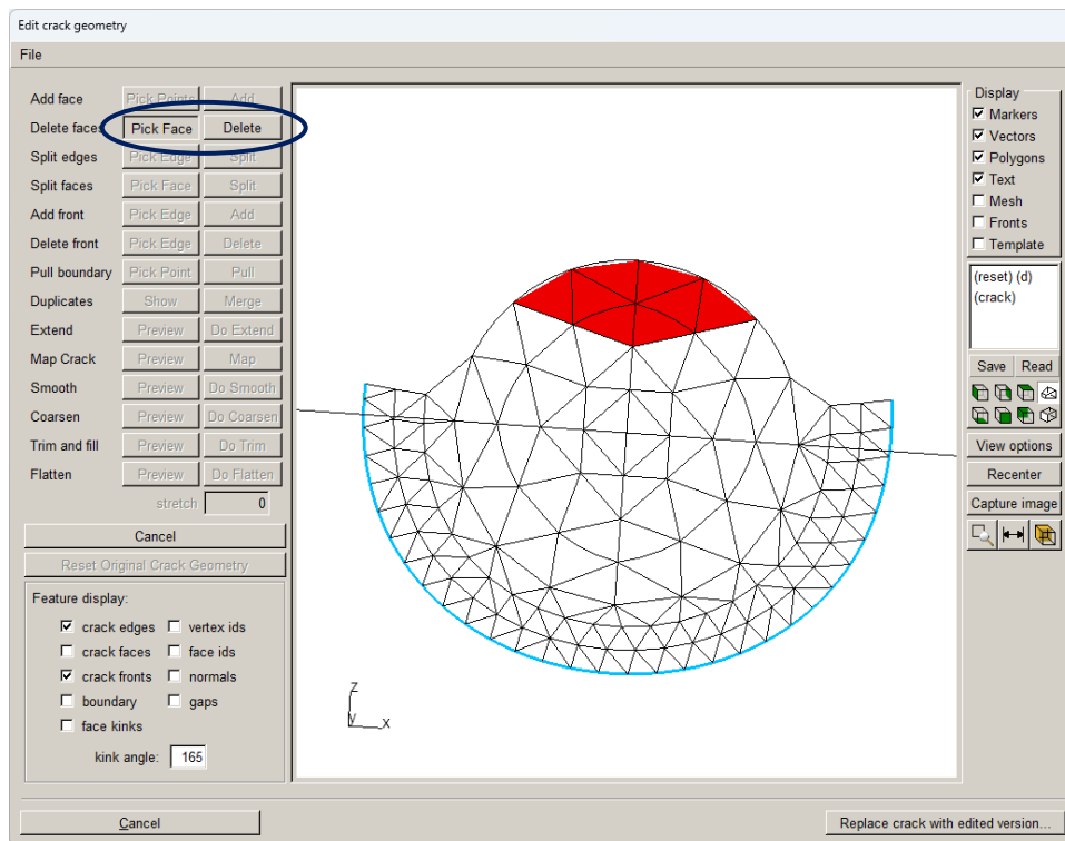
Figure 8.50a Delete face(s) from crack.
