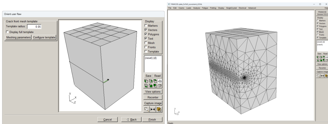
Figure 4.13 Edge crack inserted and remeshed.
