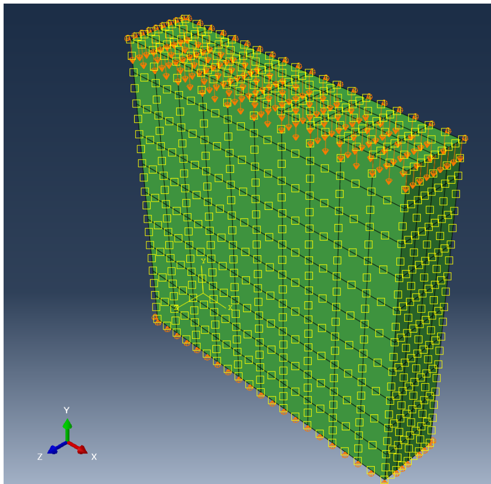
Figure 14.1 Plate with applied displacement for load step 1.
