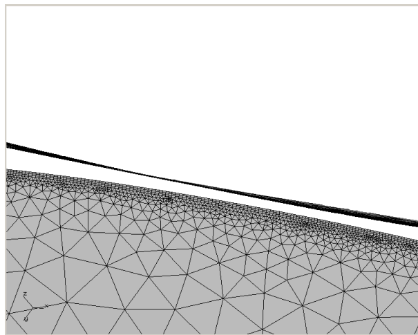
Figure 8.25 Crack surface mesh near the model back surface.
