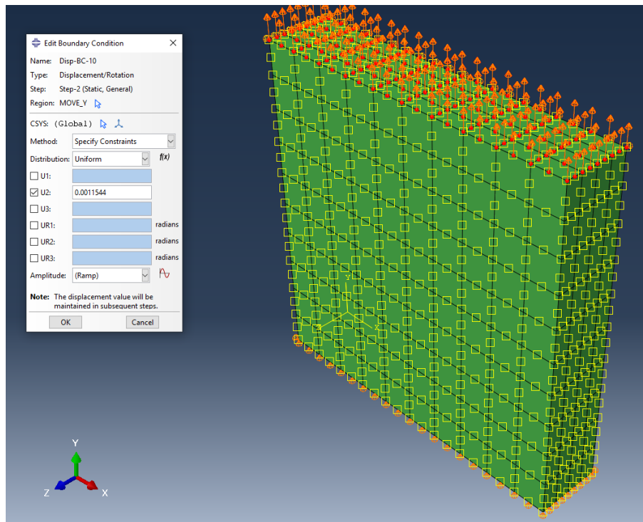
Figure 14.5 Plate model without plastic properties, showing applied displacement for load step 2.
