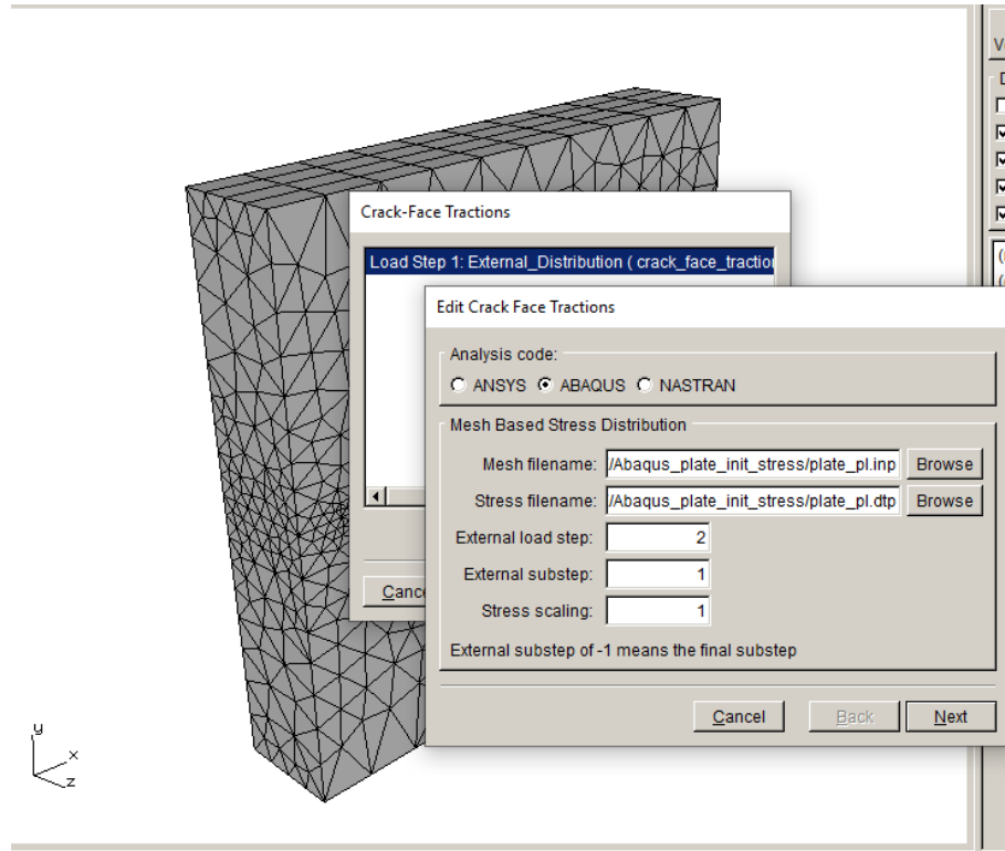
Figure 14.14 Crack face traction load step added using the plastic model and stress data.
