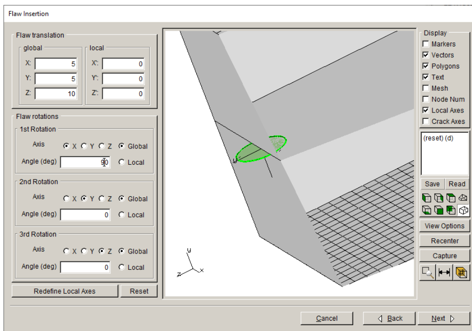
Figure 6.20 Crack is inserted in a material interface.
