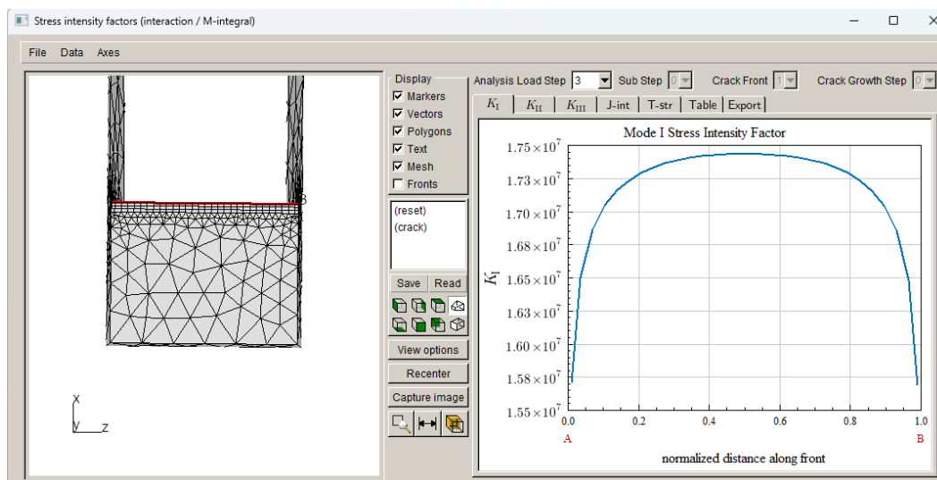
Figure 14.15c Mode I SIFs for load step 3 – the CFT loading.
