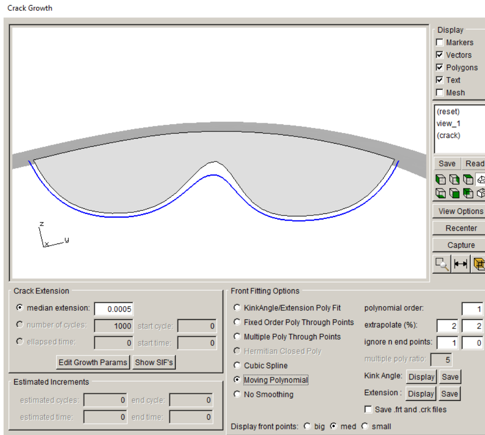
Figure 9.28 Overlap points removed during smoothing using the moving polynomial.
