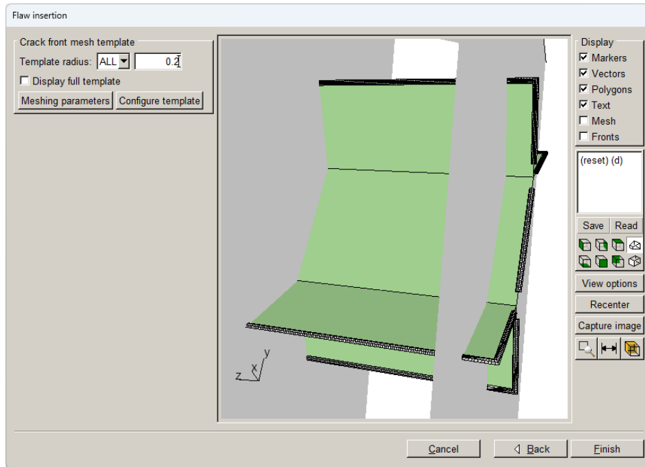
Figure 6.11 Crack front templates along the four fronts.
