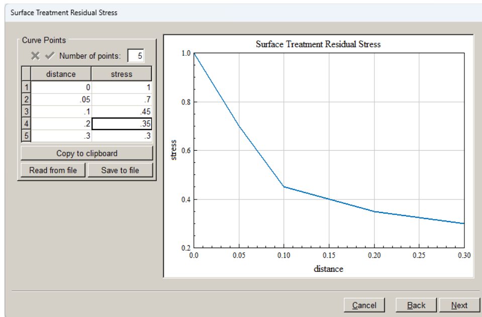
Figure 12.49 Surface treatment stress versus depth.
