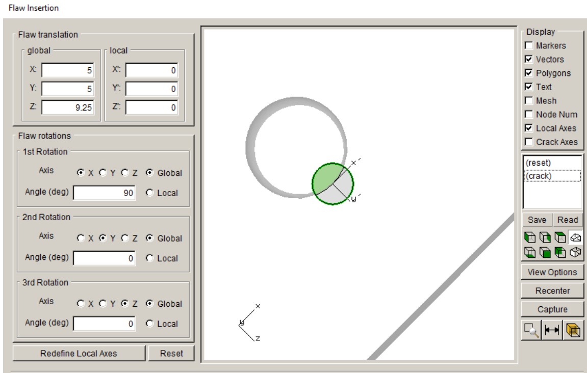
Figure 8.43 Surface penny crack inserted into a void.
