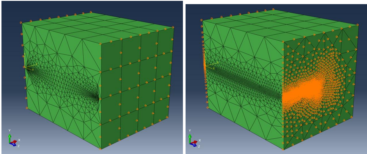
Figure 5.27 Constraints on retained mesh prior to editing, and constraints on the same surface after editing and further crack growth.
