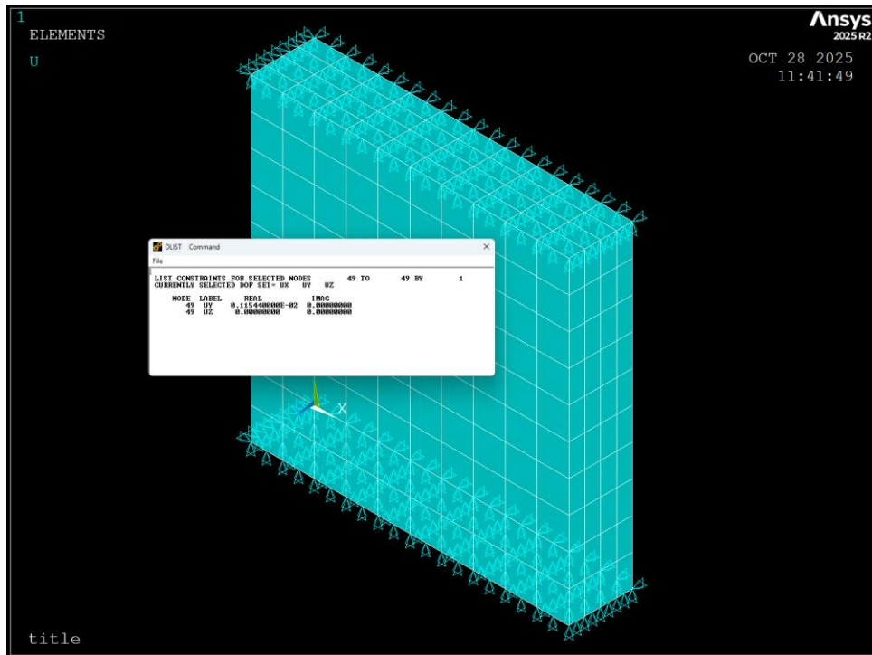
Figure 14.9 Plate model without plastic properties, showing applied displacement for load step 2.
