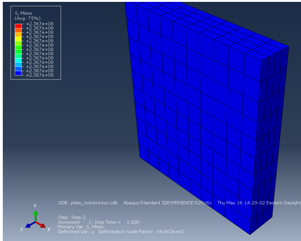
Figure 14.6 von Mises stress at the end of load step 2 for elastic plate without initial stress.
