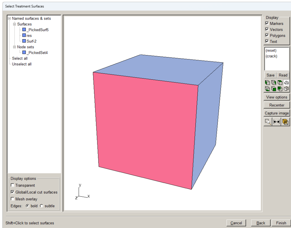
Figure 12.44 Surface treatment residual stress – full surface selected.
