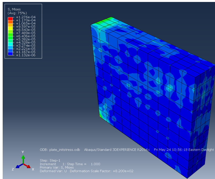
Figure 14.7b von Mises stress for load step 1 and frame 1 in the elastic plate with initial stress.
