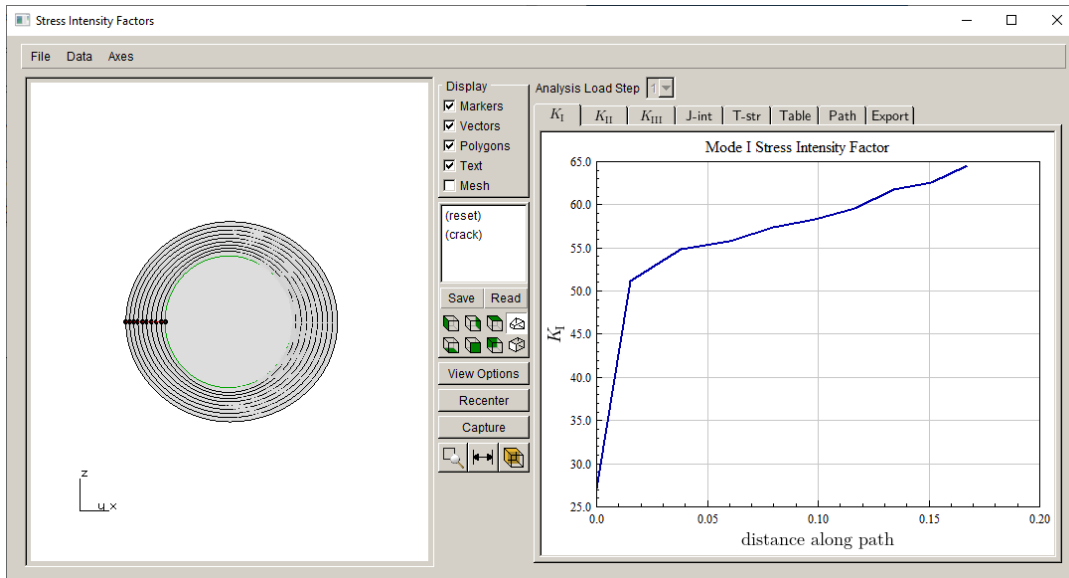
Figure 10.56 SIF history path; base simulation K_I shown.
