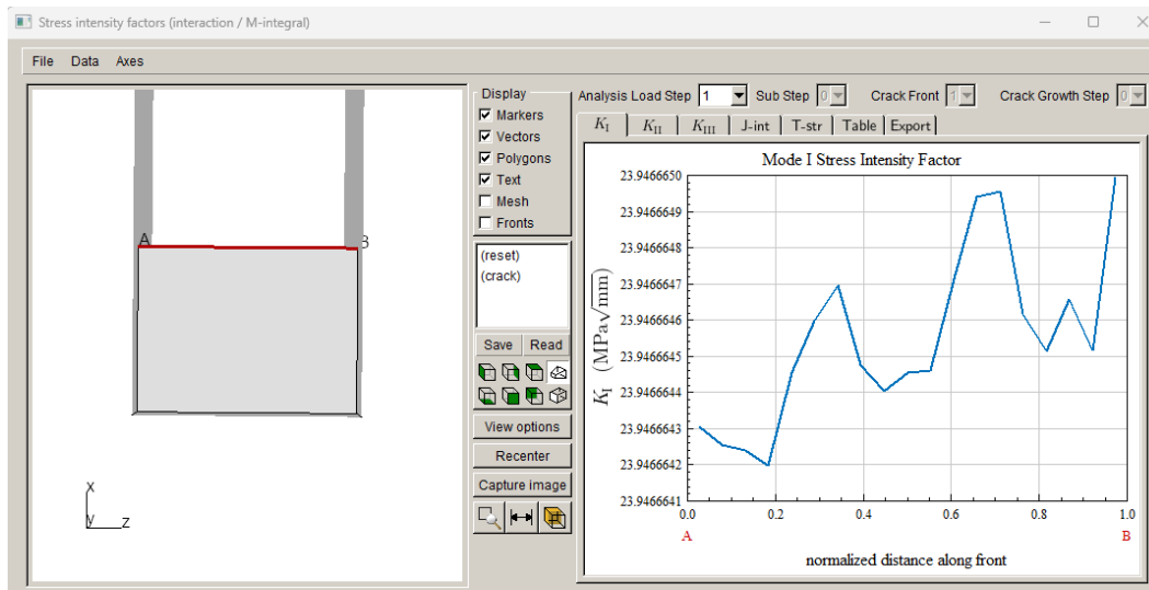
Figure 14.20a Mode I SIFs for load step 1 (final substep) – initial stress balanced.
