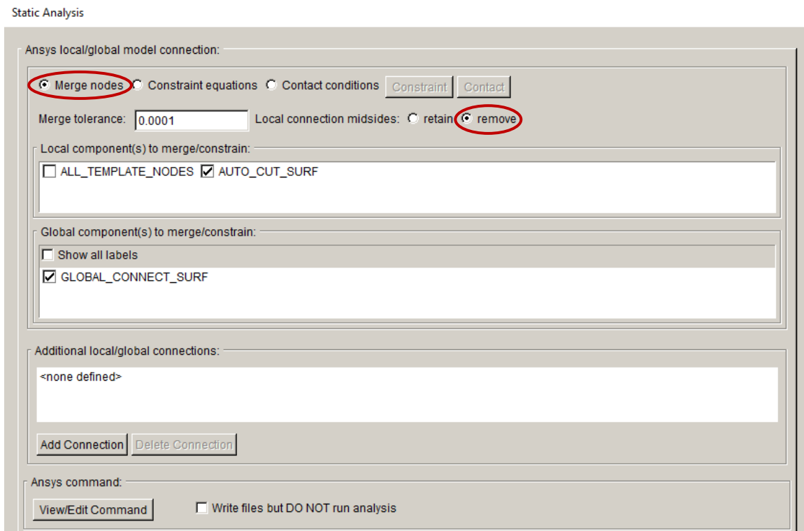
Figure 11.8 Local – global connection for a mesh with global linear elements.
