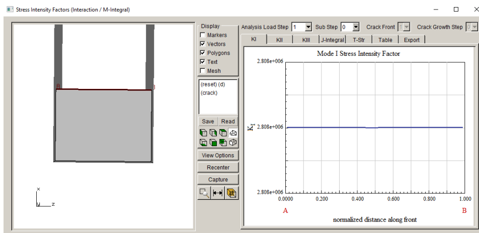
Figure 14.16a Mode I SIFs for load step 1 and frame 0 – initial stress condition.
