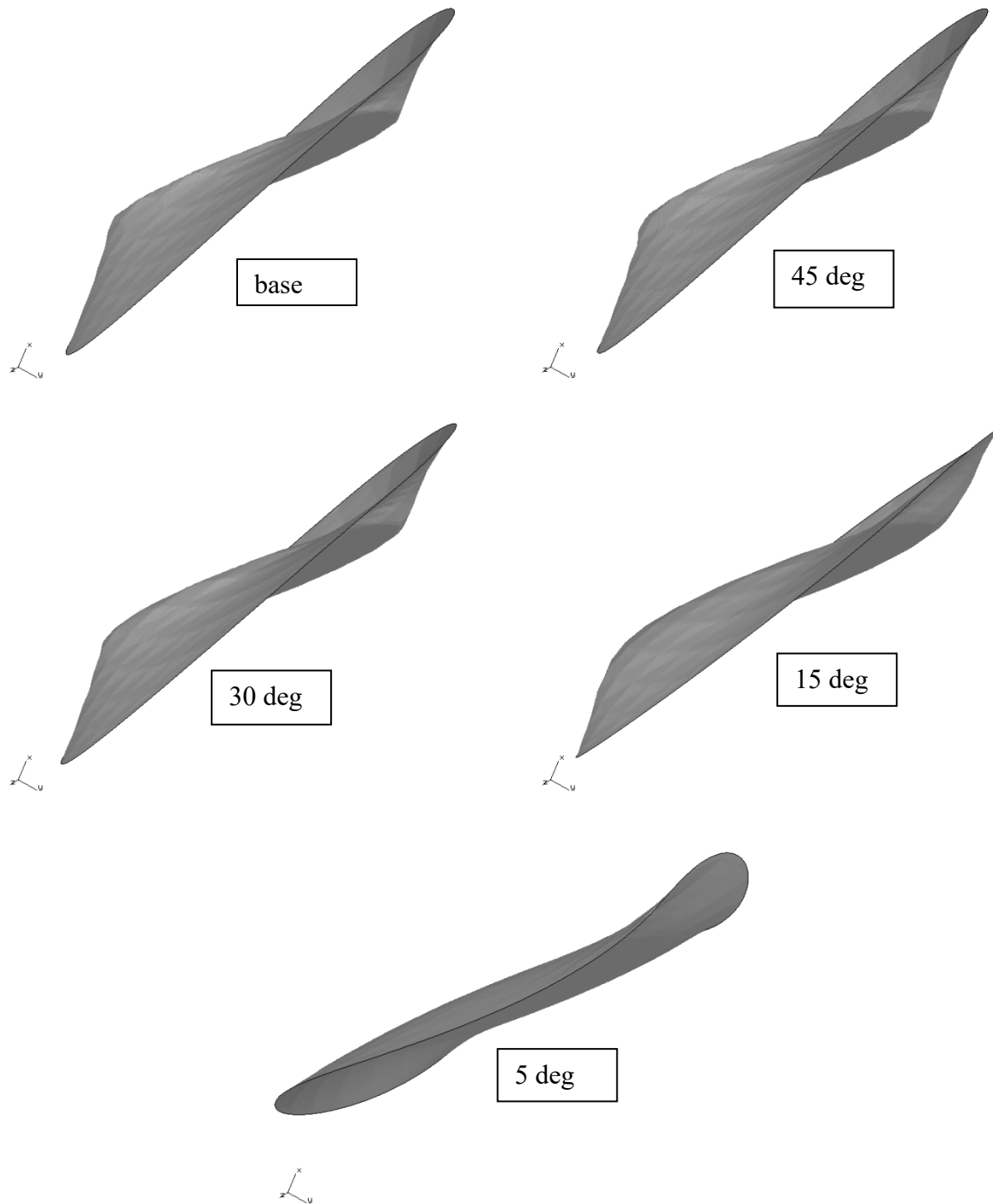
Figure 10.56 Crack shapes after 9 steps of growth for no limit (base), and then 45, 30, 15 and 5 deg kink angle limits.
