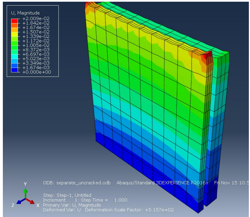
Figure 15.3 Separate plate model deformed shape.
