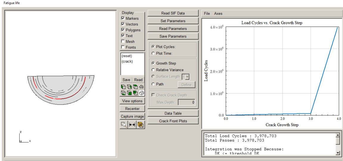
Figure 10.48 Cycle count for simple cyclic load event with missing substeps at crack step 4.
