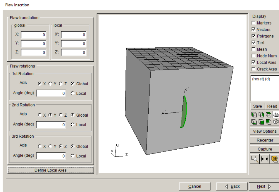
Figure 6.29 Crack is oriented in a local coordinate system.
