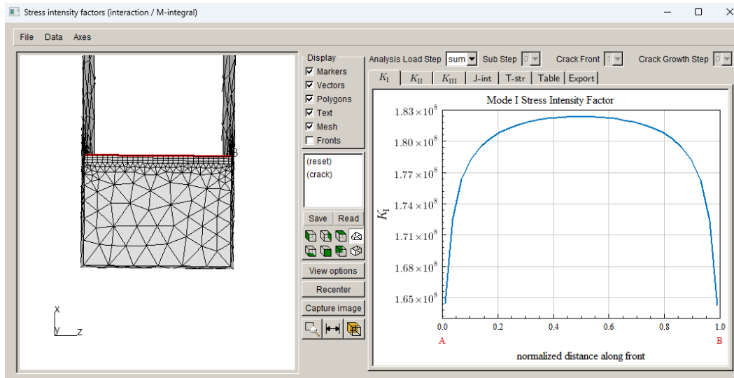
Figure 14.15d Sum of Mode I SIFs.
