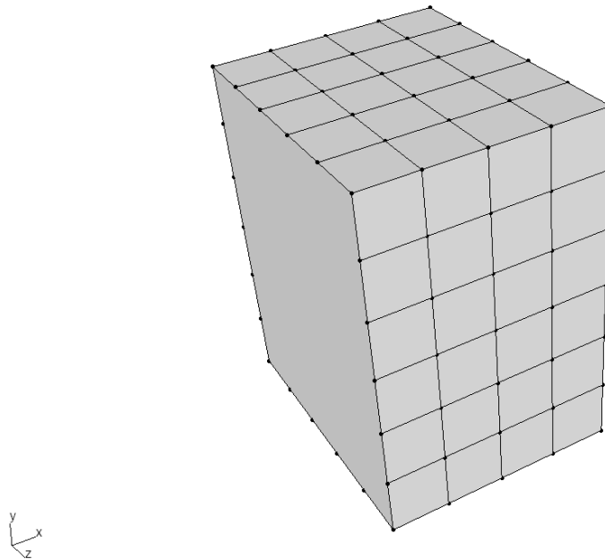
Figure 5.19 FRANC3D local model.
