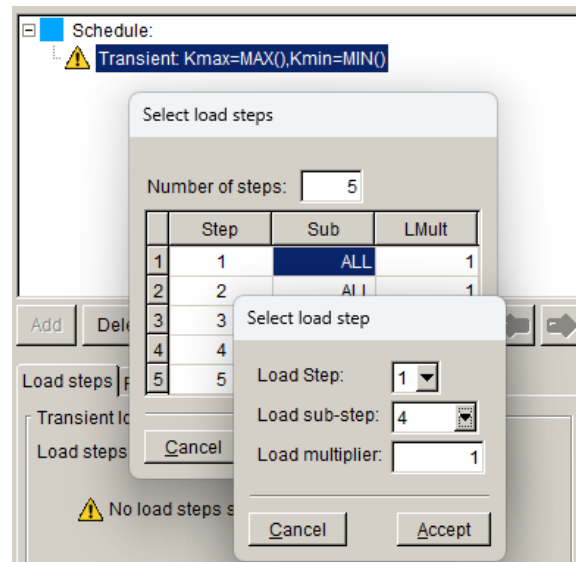
Figure 10.42 Choosing specific substeps for a load step.
