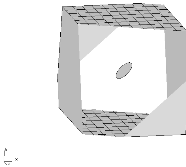
Figure 10.54 Initial 45-degree interior penny-shaped crack.
