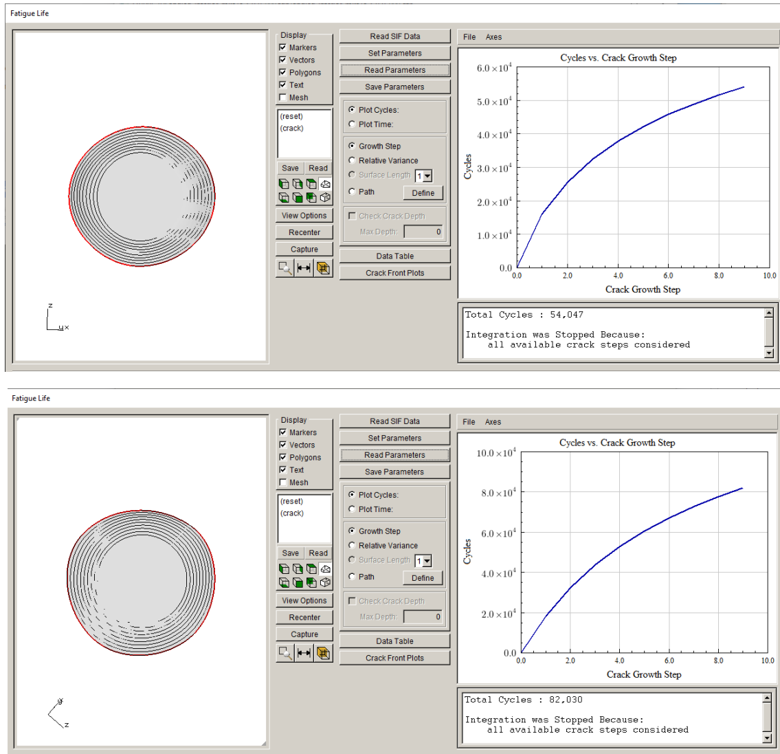
Figure 10.58 Paris model cycles for no limit (base) and then 45, 30, 15 and 5-deg limits.
