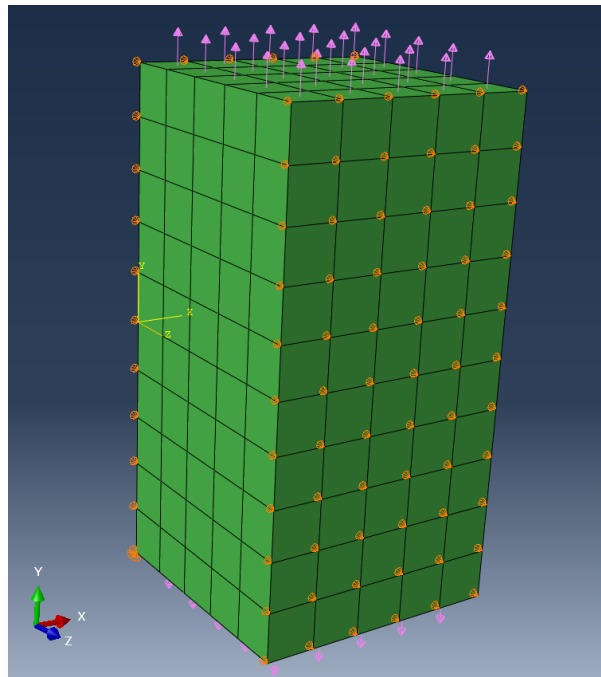
Figure 5.16 Traction and constraint applied.
