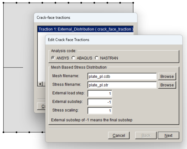
Figure 14.17 Crack face traction load step added using the plastic model and stress data.
