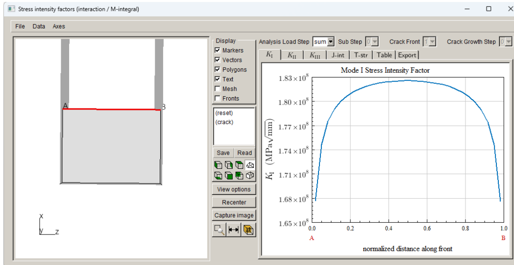
Figure 14.18d Sum of Mode I SIFs.
