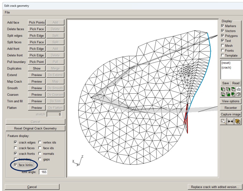
Figure 8.53 Overlapping faces produce excessive kink angles at adjacent edges.
