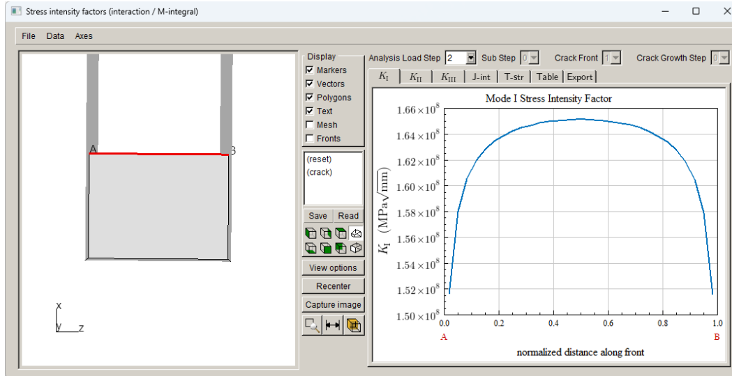
Figure 14.18b Mode I SIFs for load step 2.
