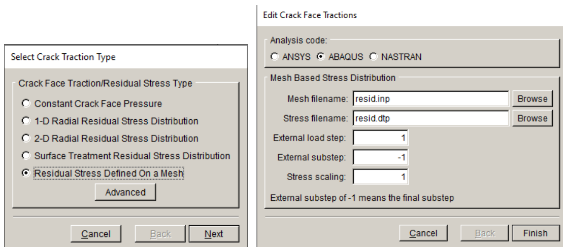
Figure 12.43 FRANC3D dialogs for mesh-based residual stress CFTs.
