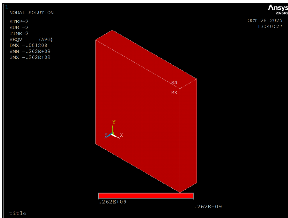
Figure 14.12 von Mises stress for load step 2 in the elastic plate with initial stress.
