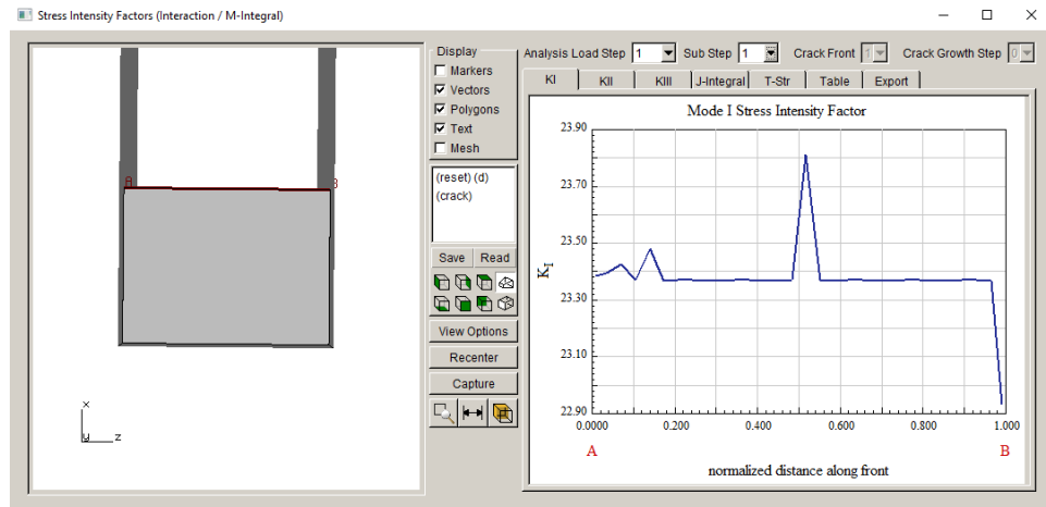
Figure 14.16b Mode I SIFs for load step 1 and frame 1 – initial stress balanced.
