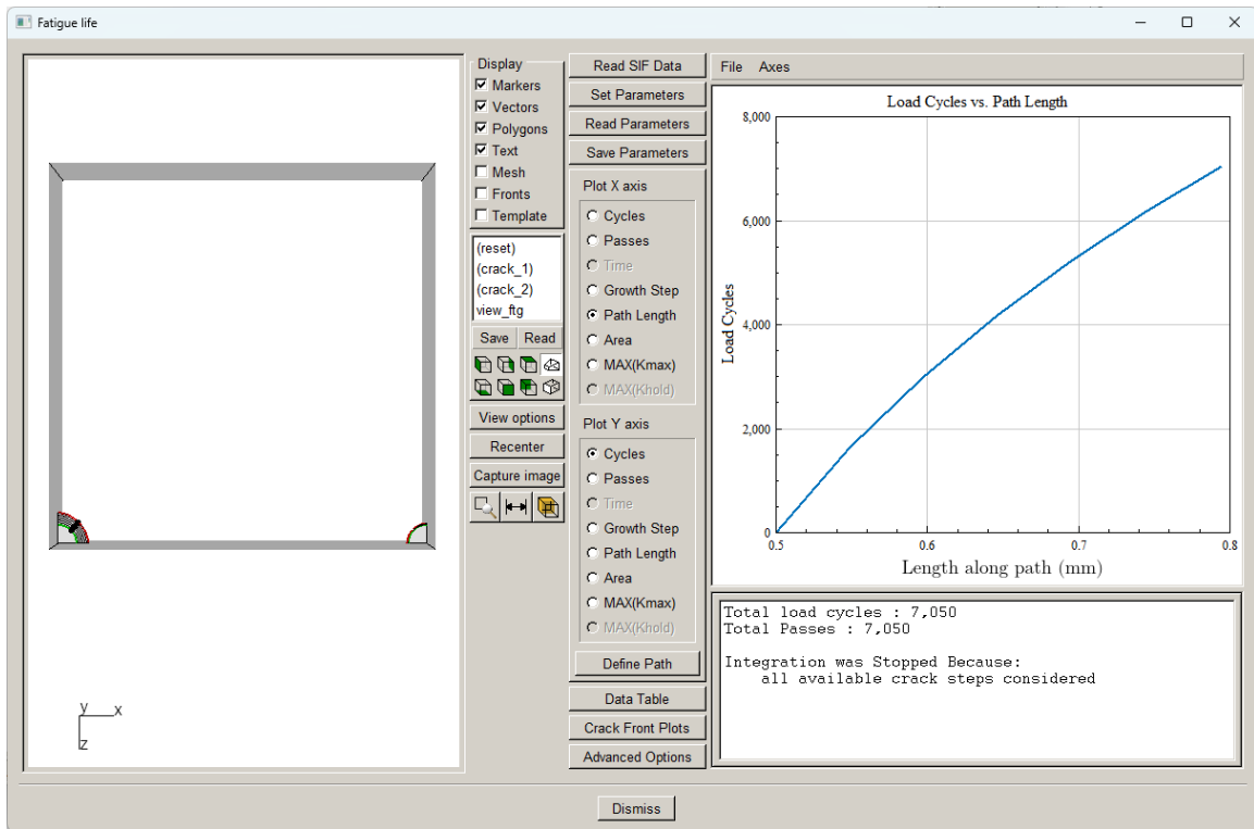
Figure 10.62 Cycles for both corner cracks with quasi-static growth.
