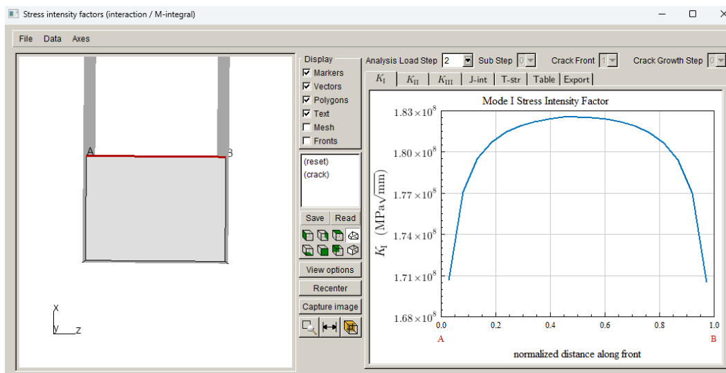
Figure 14.20b Mode I SIFs for load step 2.
