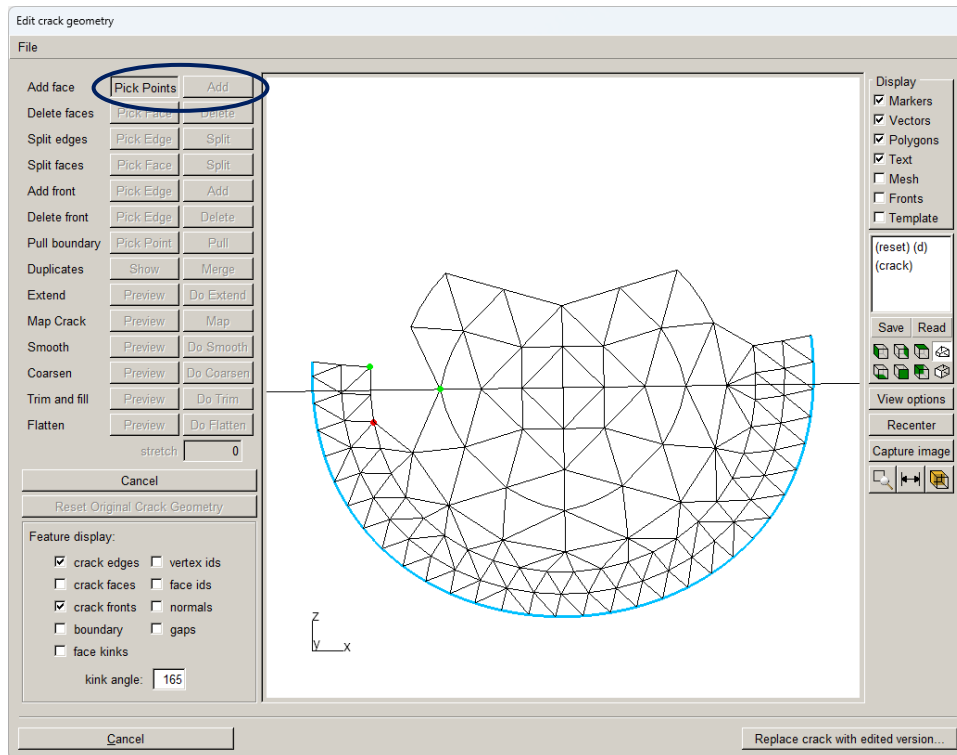
Figure 8.51a Pick points to define a new face.
