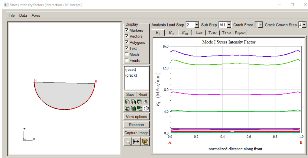
Figure 10.49 SIF plot for load step 2 for ALL substeps.
