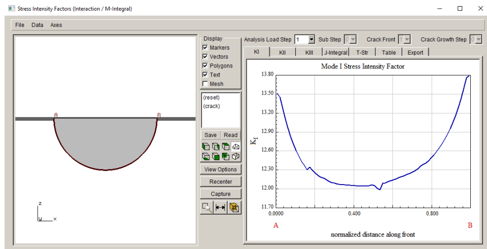
Figure 12.35b Mode I SIFs for the base load.
