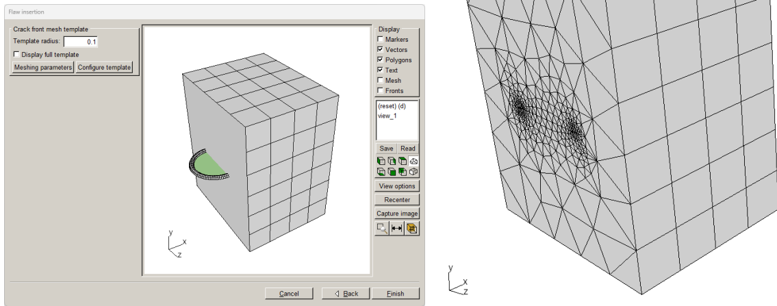
Figure 5.20 Surface half-penny crack inserted into local model.
