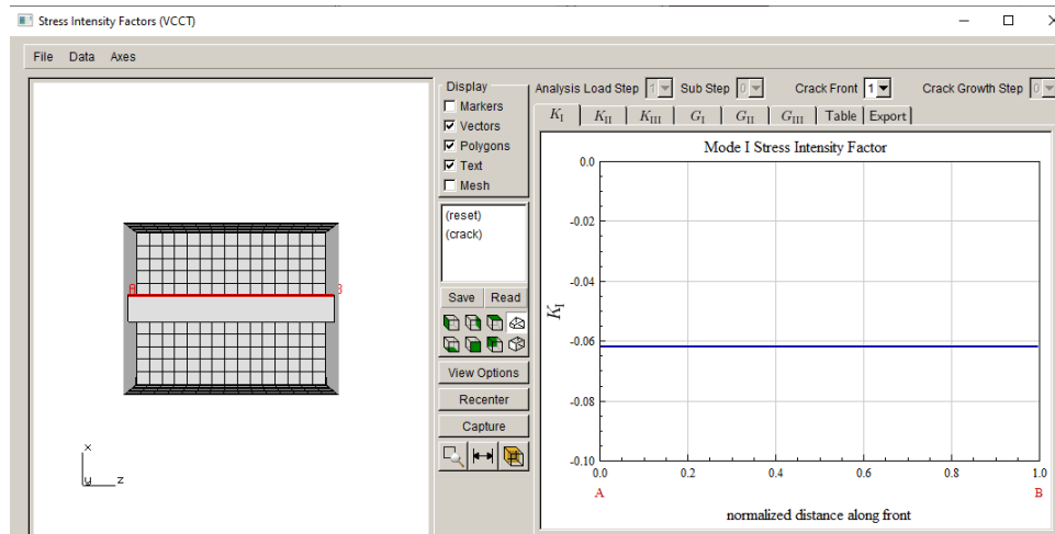
Figure 13.26 Mode I SIFs with modified template and default CFC using VCCT.
