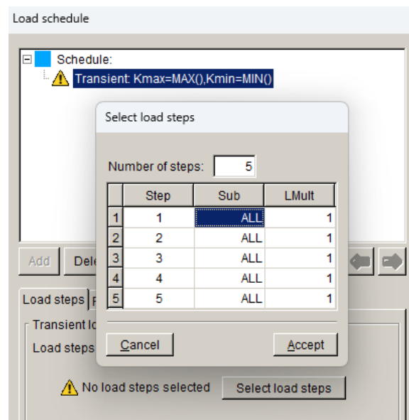
Figure 10.43 Select load steps dialog – Sub Step ID is set to ALL.
