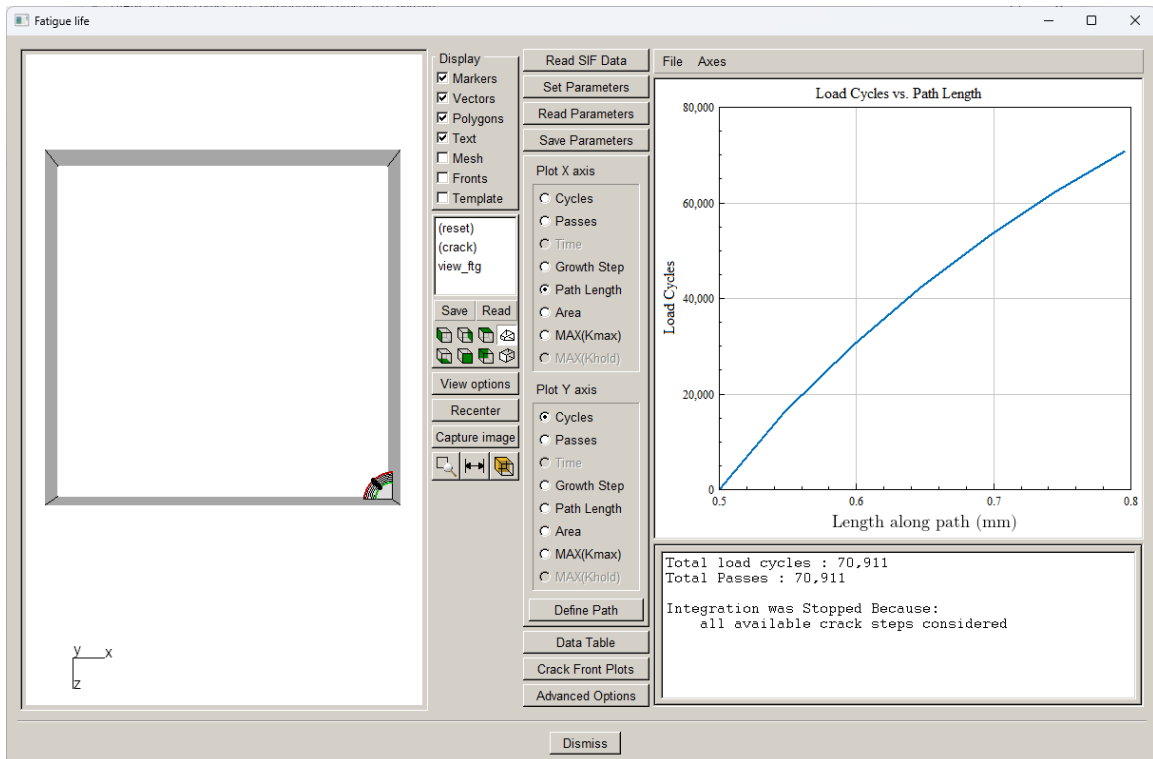
Figure 10.61 Cycles for front right corner crack.
