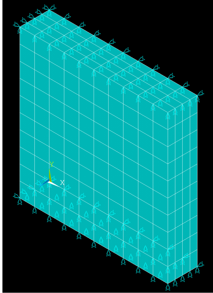
Figure 14.3 Plate with applied displacement for load step 1.
