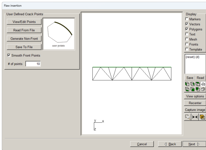
Figure 6.4 Reasonable number of front points.
