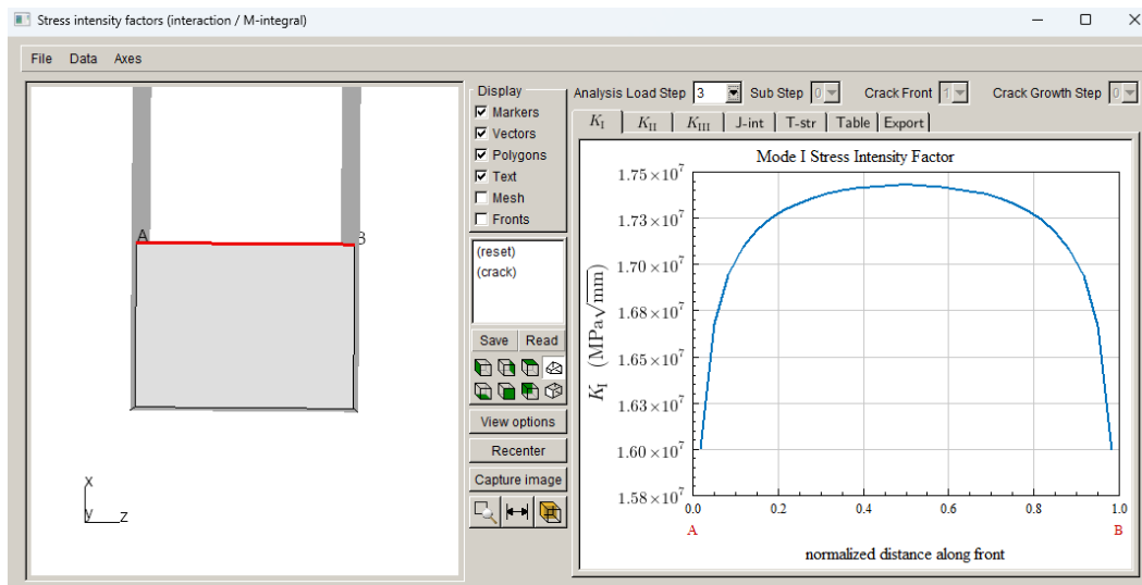
Figure 14.18c Mode I SIFs for load step 3 – the CFT loading.
