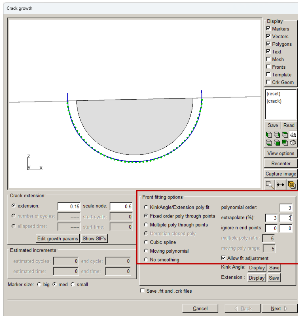
Figure 9.1 Front fitting options.
