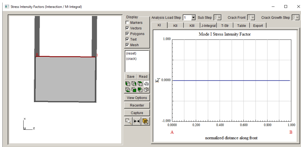
Figure 14.15a Mode I SIFs for load step 1.
