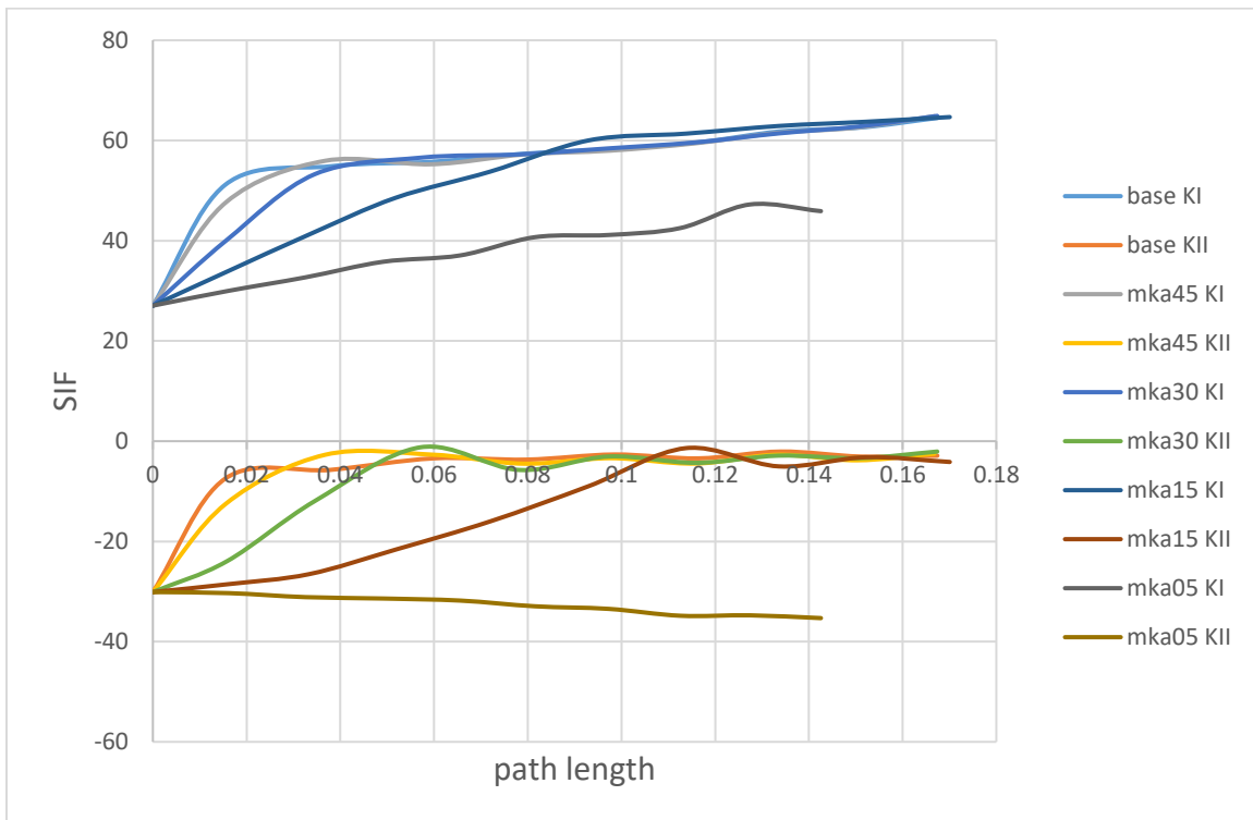
Figure 10.57 SIFs along path for various kink angle limits.
