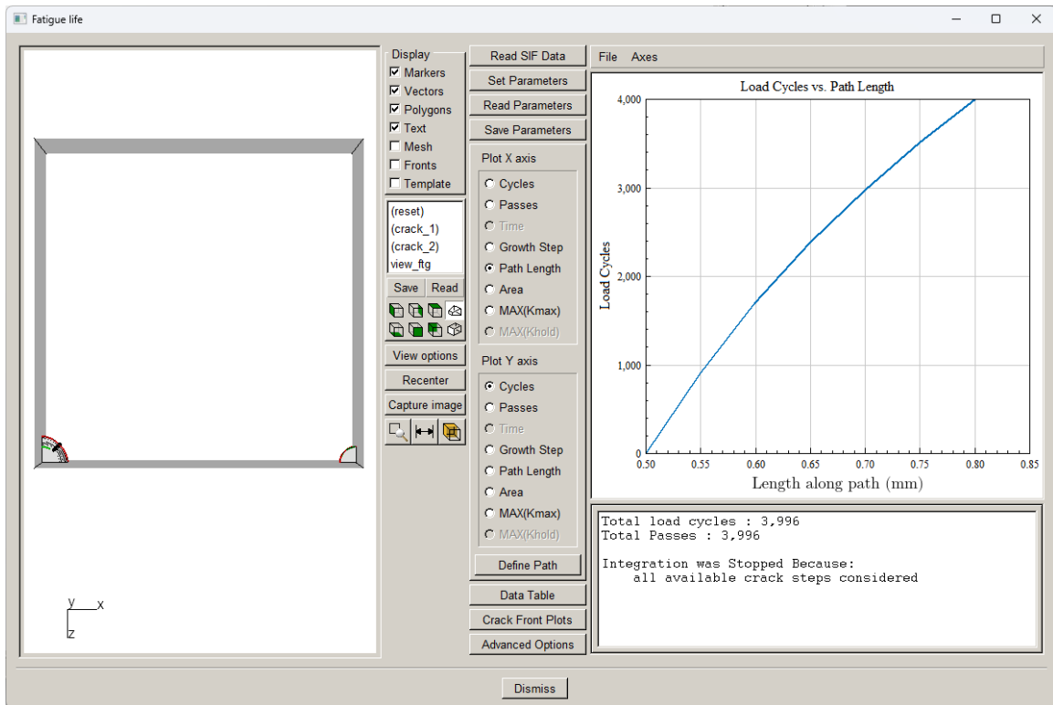
Figure 10.63 Cycles for both corner cracks with subcritical growth.
