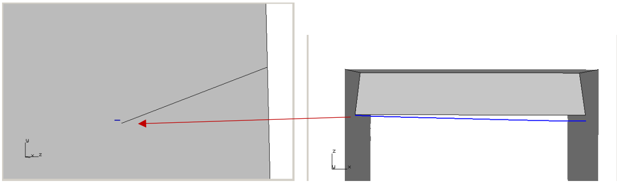
Figure 9.32 Crack front turns (kinks).
