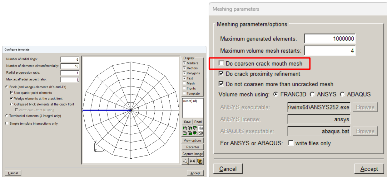
Figure 2.4 Template options (left) and meshing parameters (right); Do coarsen... is off.
