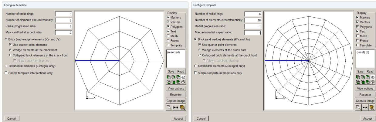
Figure 3.3 Default (left) and refined (right) crack front template settings.
