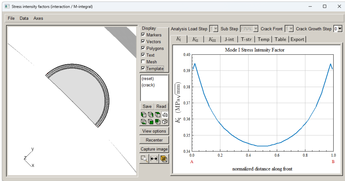
Figure 10.4 Pipe - transverse crack Mode I SIFs.
