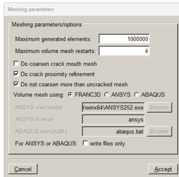
Figure 5.5 Edge crack meshing parameters.
