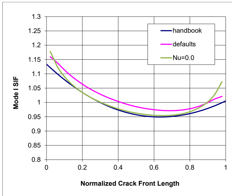
Figure 7.6 Mode I SIF for corner crack in plate with hole for Nu=0 .
