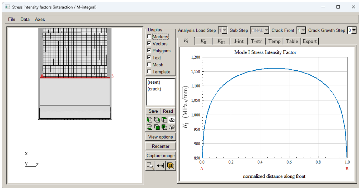
Figure 8.4 Compact tension Mode I SIF with \nu=0.33 .
