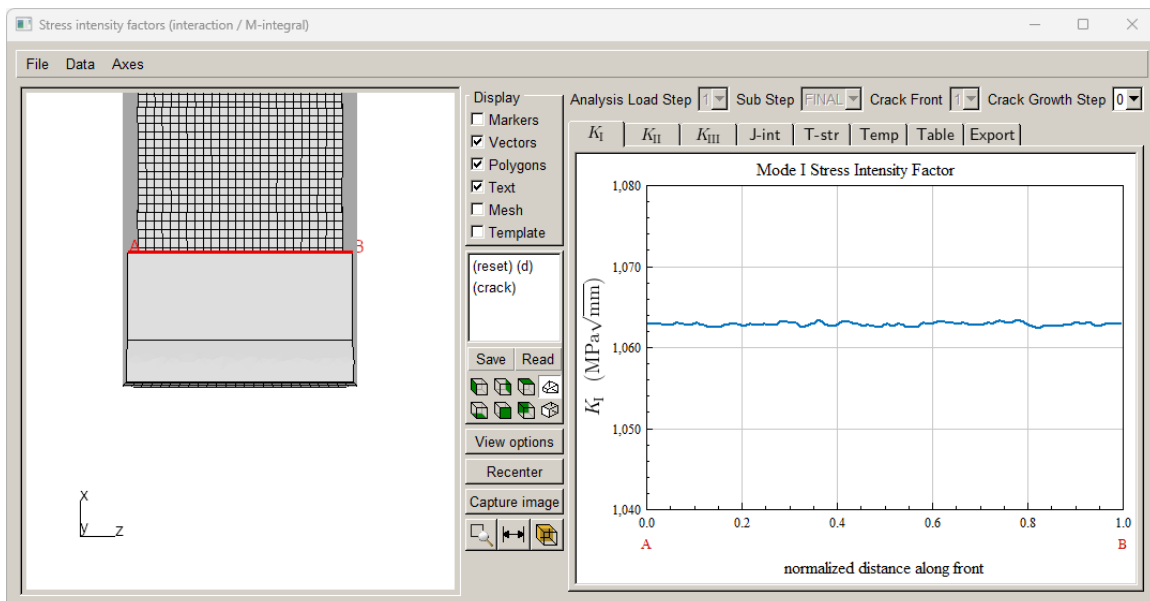
Figure 8.5 Compact tension Mode I SIF with \nu=0 .
