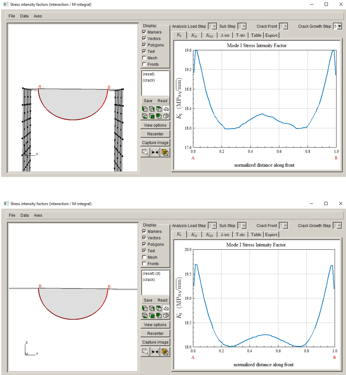
Figure 2.84 Step 5 Mode I SIFs for the original submodel analysis (top) compared with the new results using the full model (bottom).
