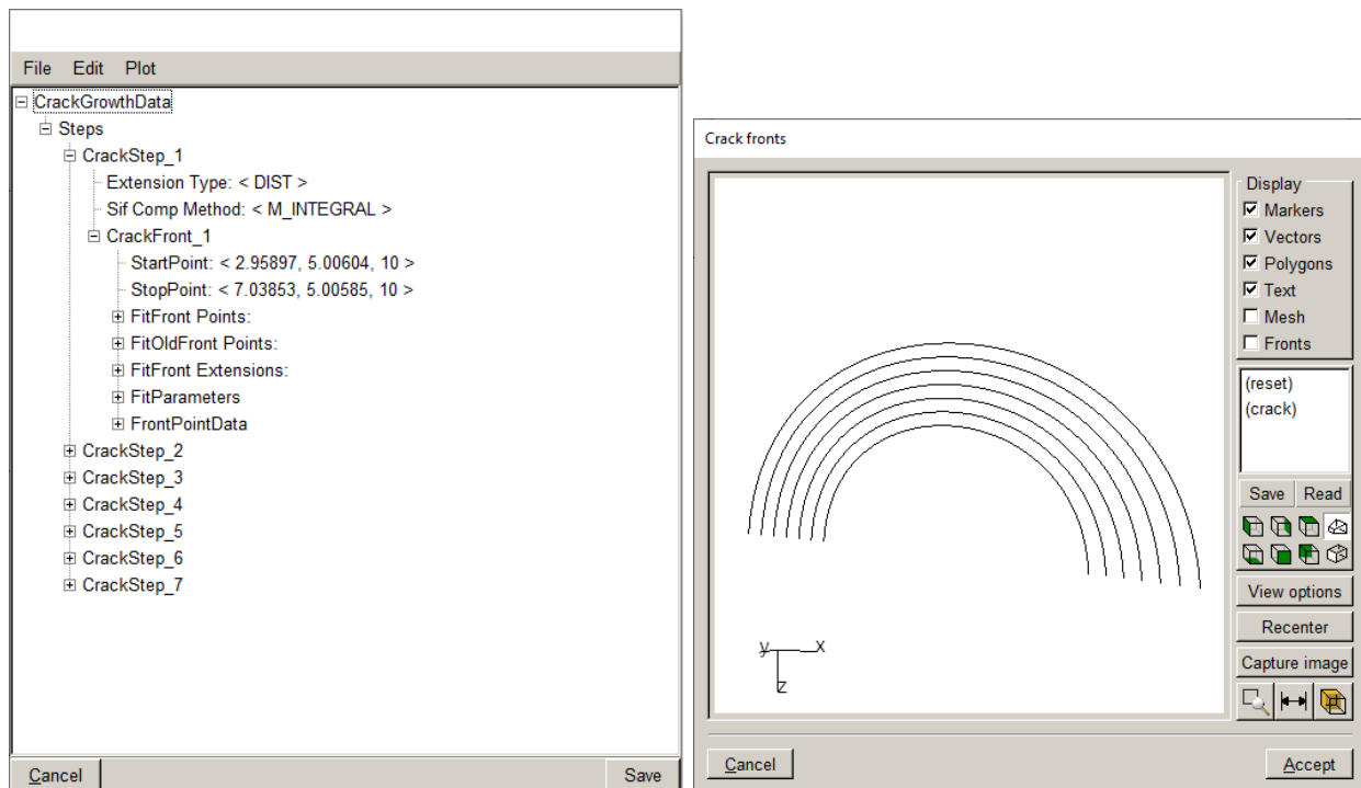
Figure 2.89 Create Growth History dialog – full model fronts 5-11.
