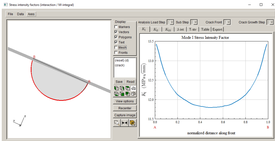
Figure 2.39 Stress Intensity Factor display
