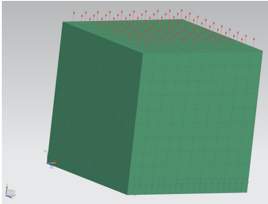
Figure 2.1 NASTRAN cube with brick element mesh and boundary conditions.
